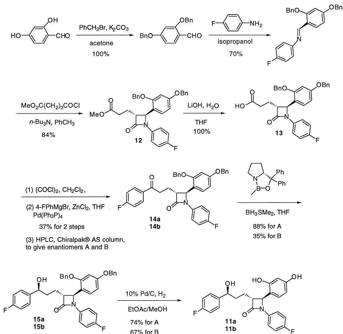
Scheme 2. Preparation of 11a and 11b .
