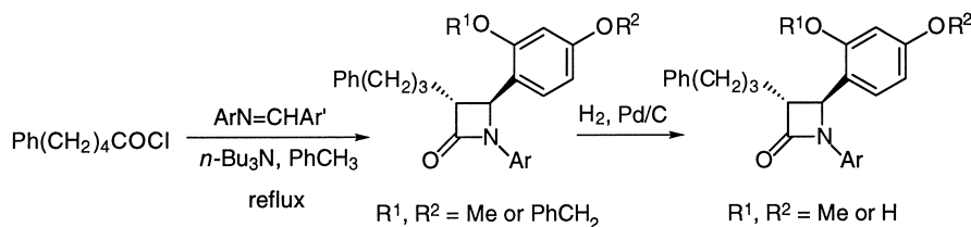
Scheme 1. Preparation of trans -2-azetidinones.
